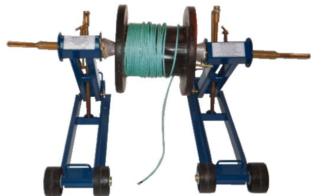
DRUM JACK NO.2 with Ball Bearing Head
