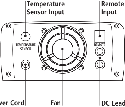
IC2500W
