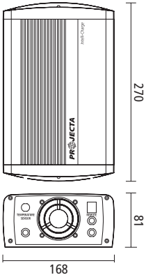
IC5000
